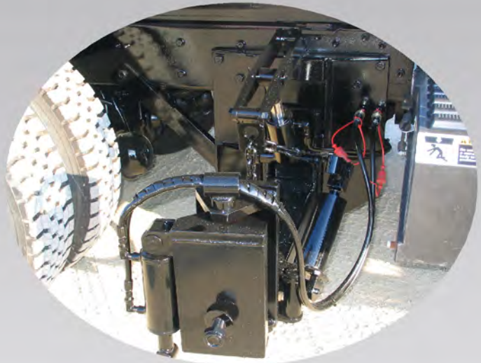
FOLD OUT WING MOUNTED ON TRUCK CHASSIS
